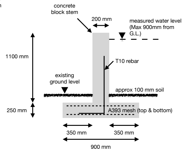
Retaining Wall. Type B Section
